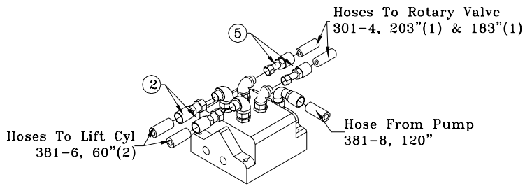
Valve Bank
